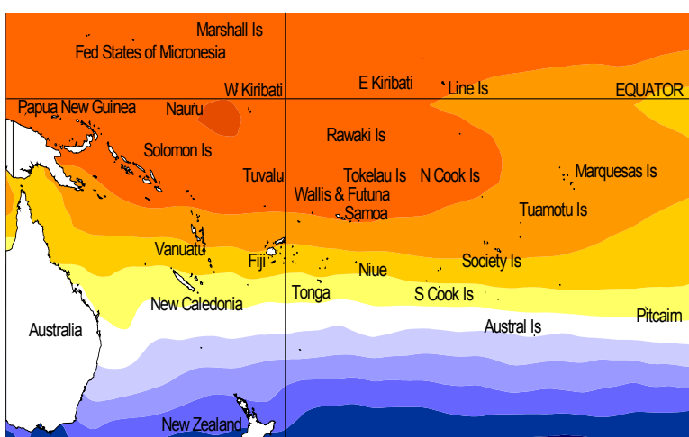
Mean sea surface temperatures (°C) for August 2009
