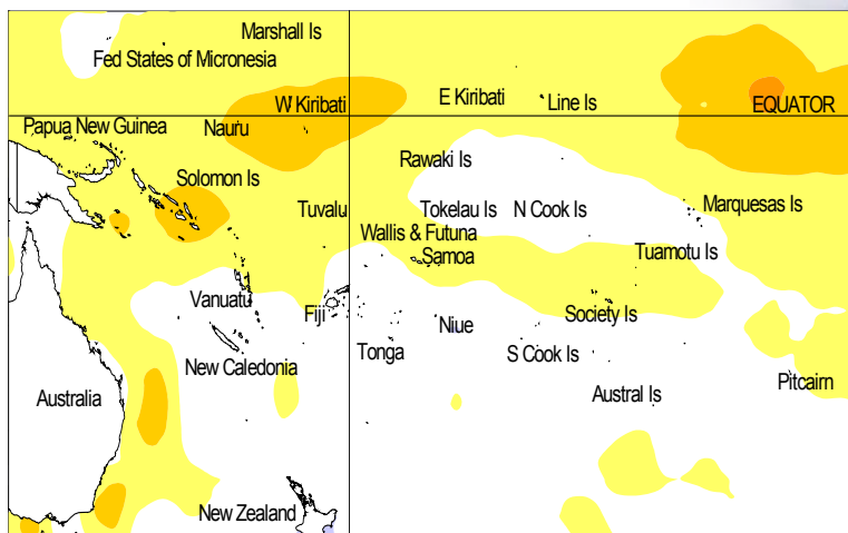
Sea surface temperature anomalies (°C) for August 2009
