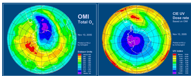
Figure 3. Total ozone measured by satellite on November 10, 2005 (left panel) showing the ozone hole displaced towards the South Atlantic, and estimated peak surface UVI calculated from the same measurements (right panel).
