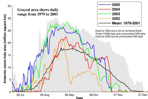
Figure 1. The area of the Antarctic ozone hole (total ozone < 220 DU) as a function of time for several years. The 2005 hole is shown by the blue line and 2002-2004 with lines of other colours. The range and mean size of earlier holes are also shown.
