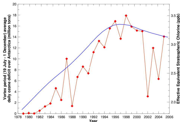
Figure 2. A measure of Antarctic ozone hole severity, the average mass of depleted ozone from July to December, diamond symbols, left axis) and an estimate of the amount of chlorine and bromine in the stratosphere, effective equivalent stratospheric chlorine (smooth curve, right axis).
