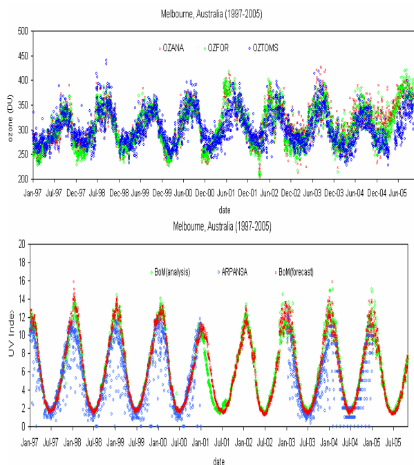
Figure 2. Melbourne 1997-2005; (top) total ozone amount Model (OZAN-OZFOR) and TOMS and (bottom) UV Index BoM Model (analysis and forecast) and ARPANSA measurements.
