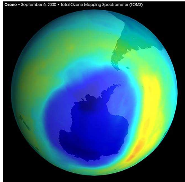
Figure 1. Total Ozone Mapping Spectrometer (TOMS) image showing the ozone hole on 6 September 2000, extending onto the southern tip of South America.
