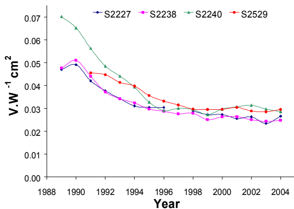
Figure 1. Average irradiance responsivity from 280 nm to 330 nm for each year of calibration for four of the six radiometers. As can be seen there is a reduction in the responsivity over this period, the rate of which has recently decreased. In addition, there is agreement between the calibrations using the Rhodamine B and silicon photodiode reference sensors (1996 to 1998).
