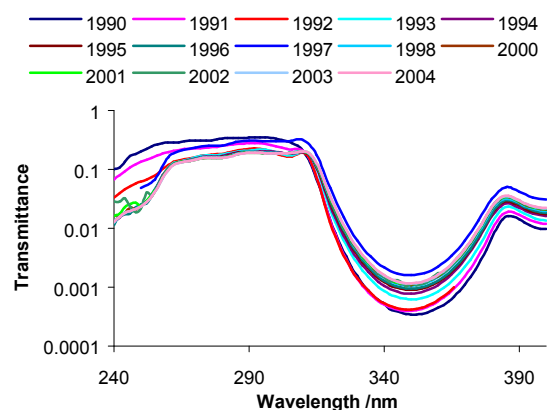
Figure 2. Spectra of filter transmittance for radiometer S2238 from 1990 to 2004. With the transmittance displayed on a logarithmic scale the change in the transmittance slope between 320 nm and 340 nm is more easily seen.
