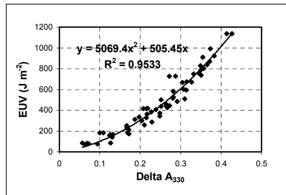
Figure 1. Dose-response of polysulphone film showing \Delta A_{330} versus YES UVB-1 pyranometer erythematous UV dose.
