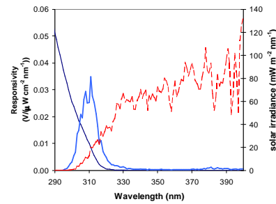
Figure 1 Graph of a) the spectral response of the Auckland radiometer in 2004 (solid line) (similar to the erythemal action spectrum); b) a typical solar spectrum with ozone column = 300 DU (dashed line); c) the product of a) and b) (thick solid line).
